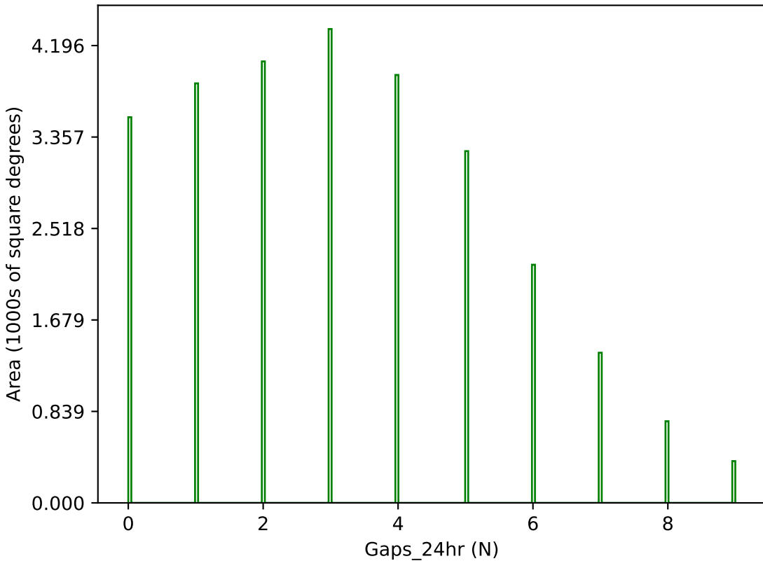
too_combined_s1.0_v3.4_10yrs g band: Gaps_24hr
