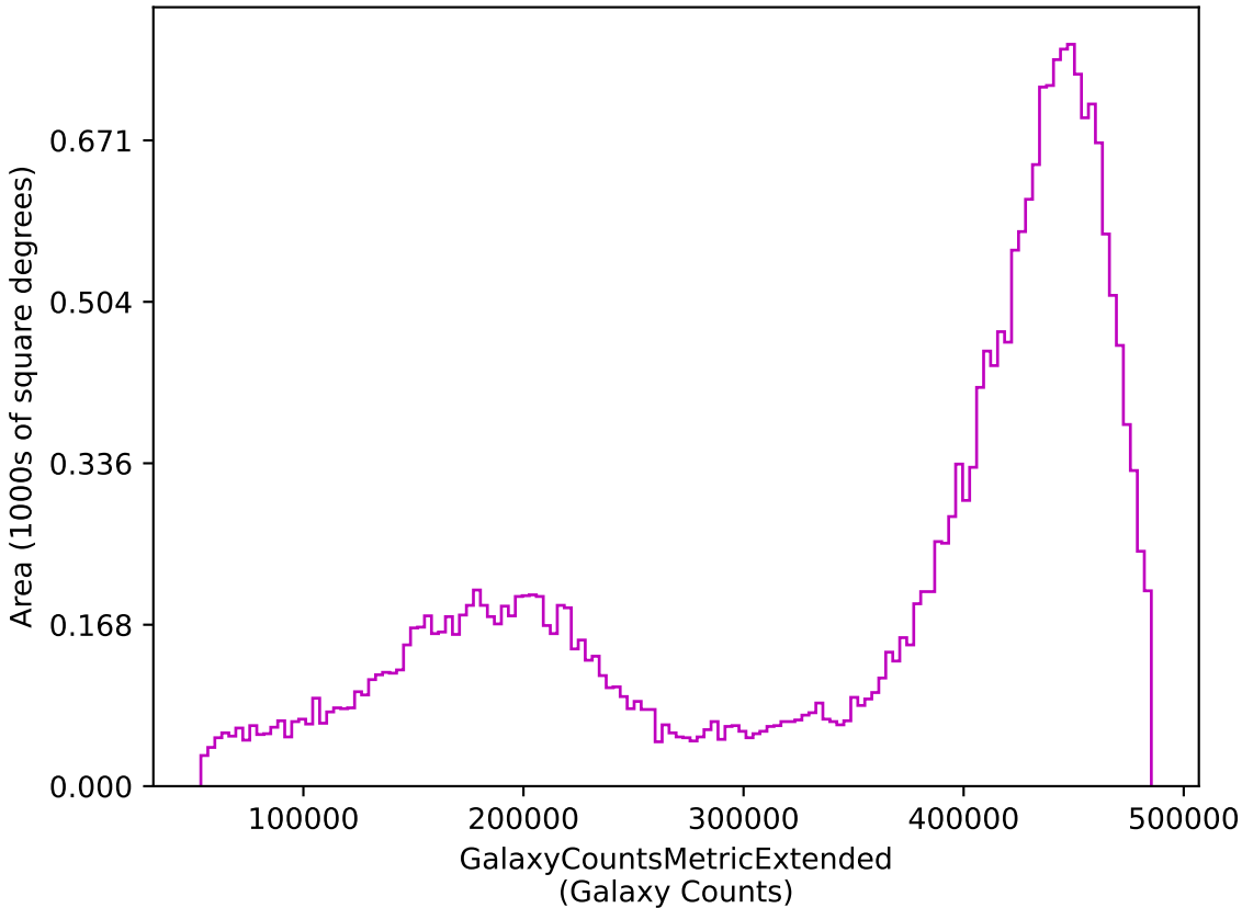
too_combined_s1.0_v3.4_10yrs z: GalaxyCountsMetricExtended
