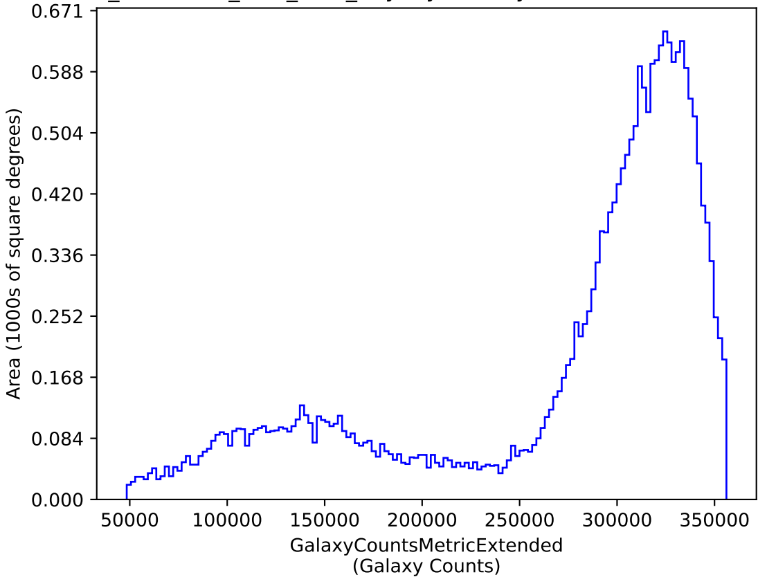
too_combined_s1.0_v3.4_10yrs y: GalaxyCountsMetricExtended
