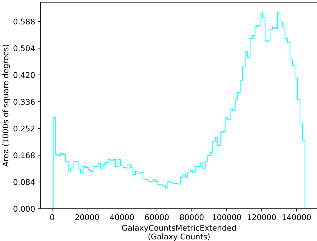
too_combined_s1.0_v3.4_10yrs u: GalaxyCountsMetricExtended
