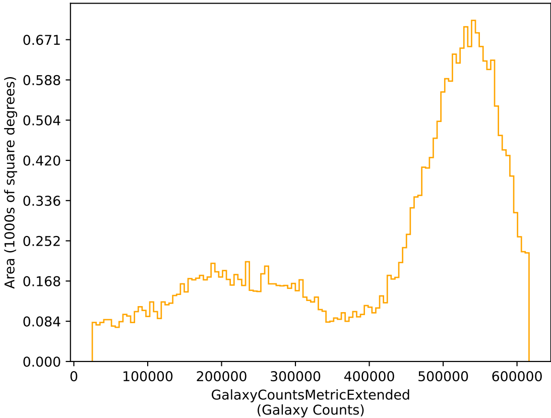
too_combined_s1.0_v3.4_10yrs r: GalaxyCountsMetricExtended
