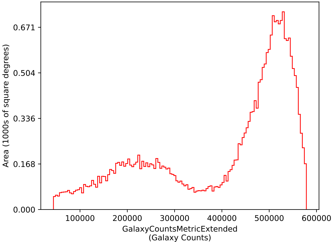
too_combined_s1.0_v3.4_10yrs i: GalaxyCountsMetricExtended
