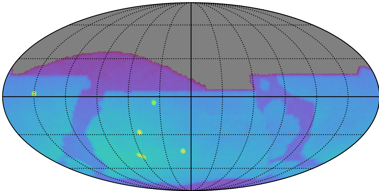
too_combined_s1.0_v3.4_10yrs : Brown Dwarf, L4
