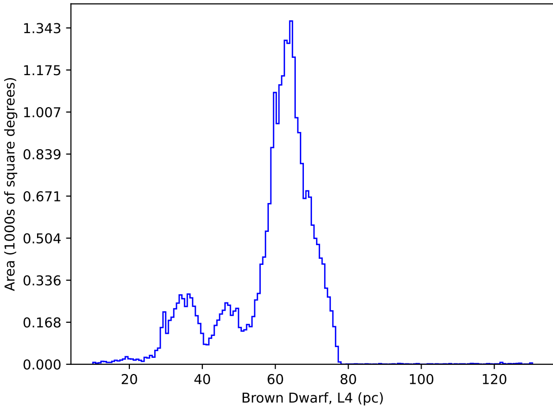
too_combined_s1.0_v3.4_10yrs : Brown Dwarf, L4
