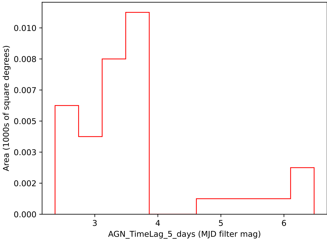
too_combined_s1.0_v3.4_10yrs i band: AGN_TimeLag_5_days
