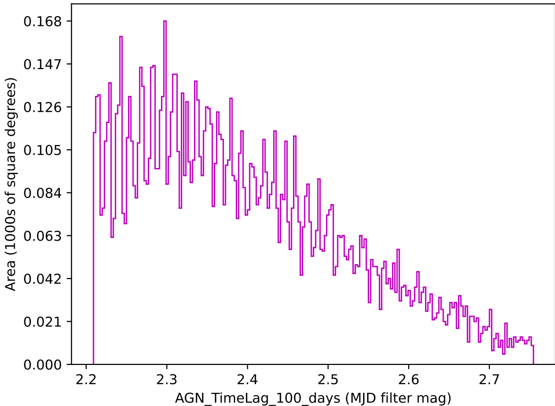
too_combined_s1.0_v3.4_10yrs z band: AGN_TimeLag_100_days
