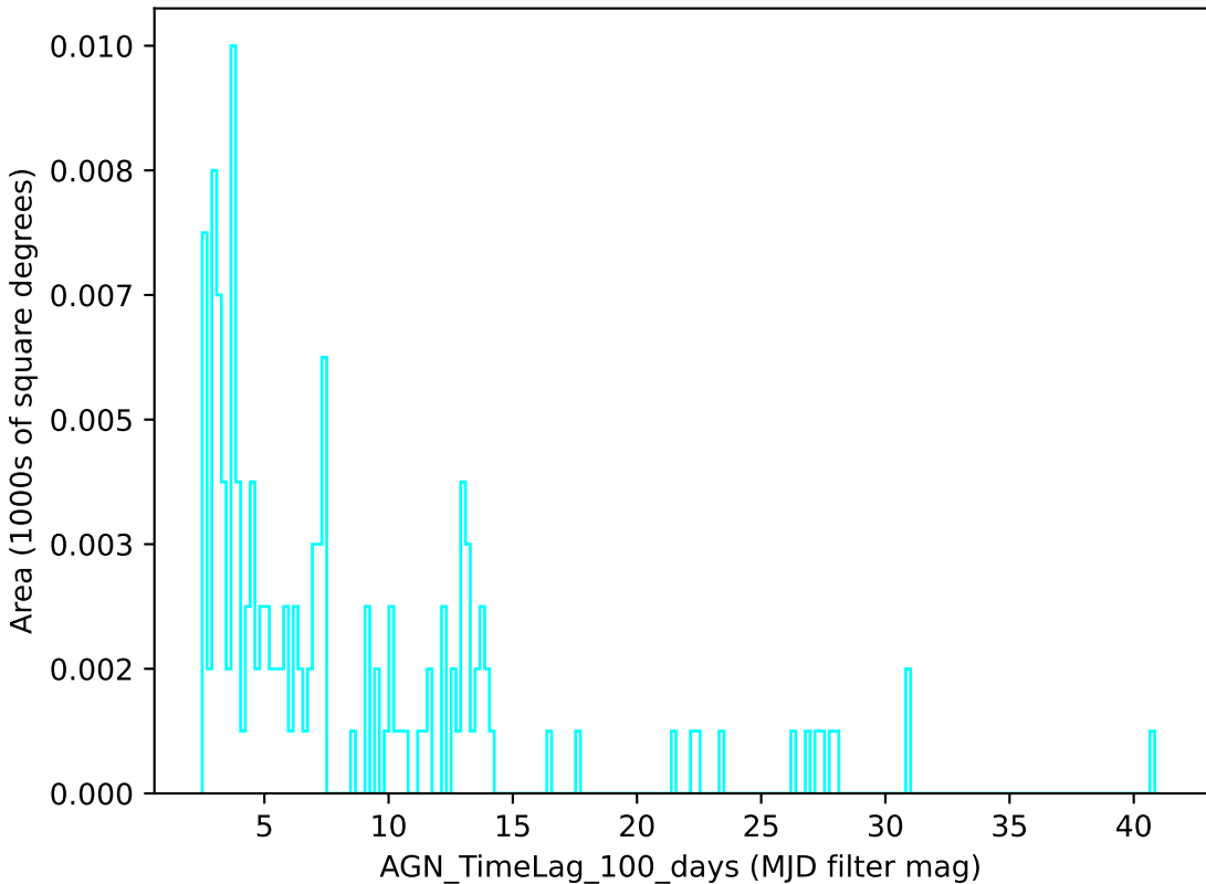
too_combined_s1.0_v3.4_10yrs u band: AGN_TimeLag_100_days
