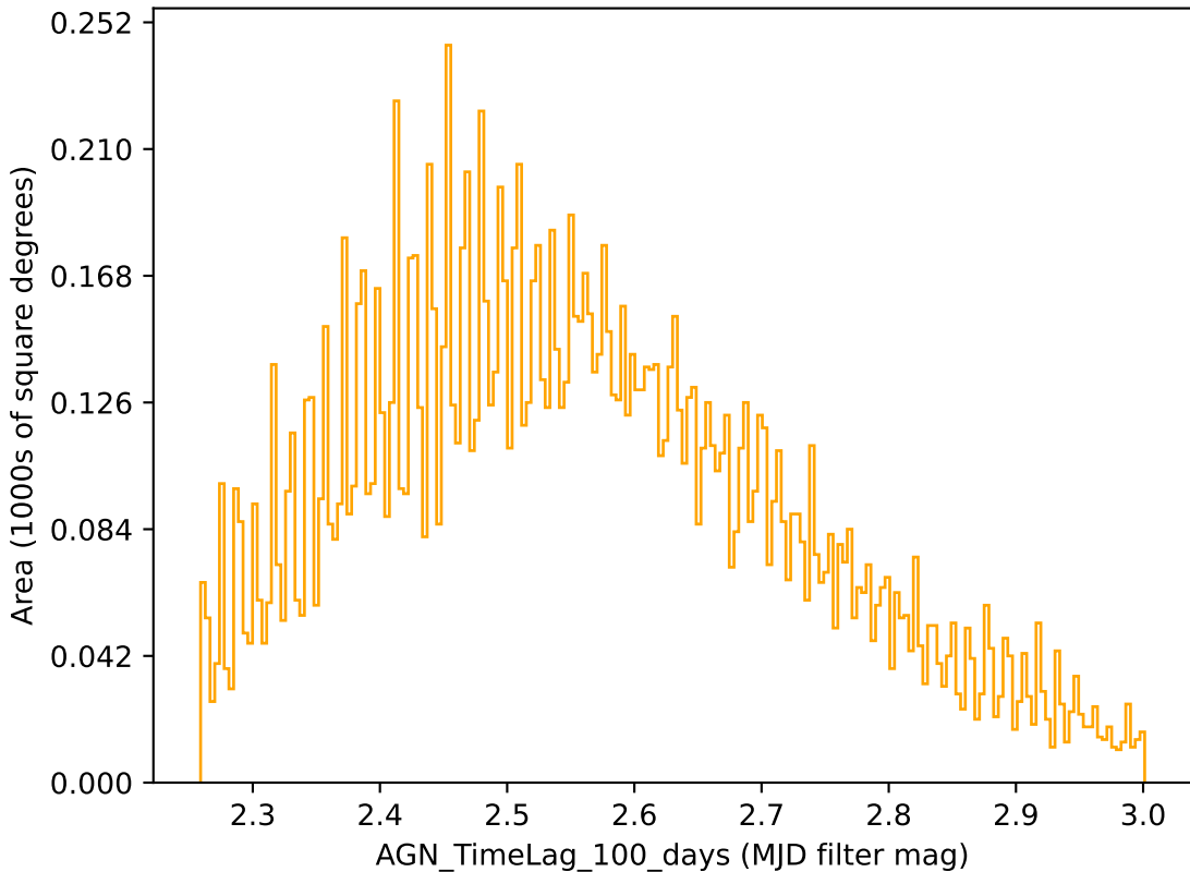
too_combined_s1.0_v3.4_10yrs r band: AGN_TimeLag_100_days
