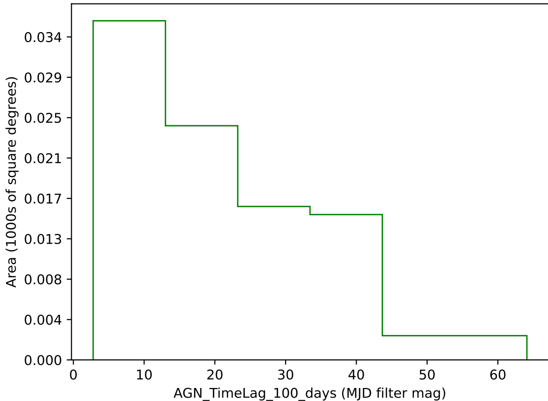
too_combined_s1.0_v3.4_10yrs g band: AGN_TimeLag_100_days
