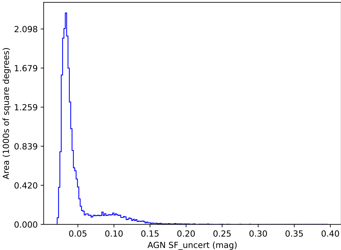
too_combined_s1.0_v3.4_10yrs y band: AGN SF_uncert
