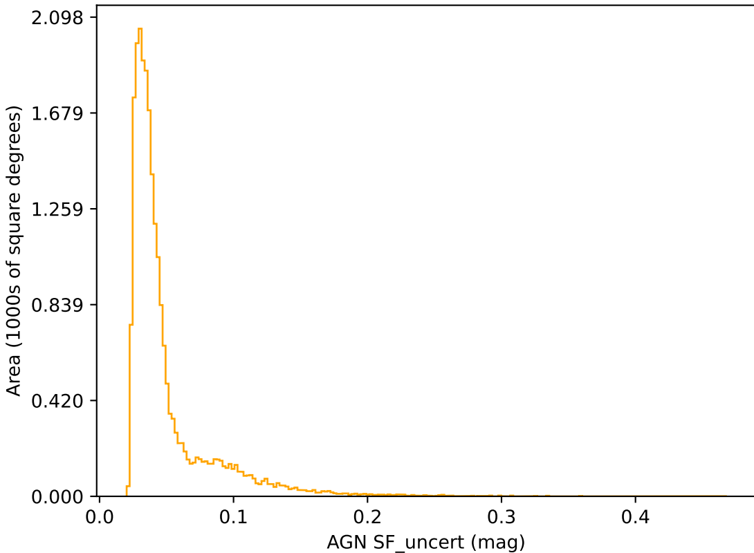
too_combined_s1.0_v3.4_10yrs r band: AGN SF_uncert
