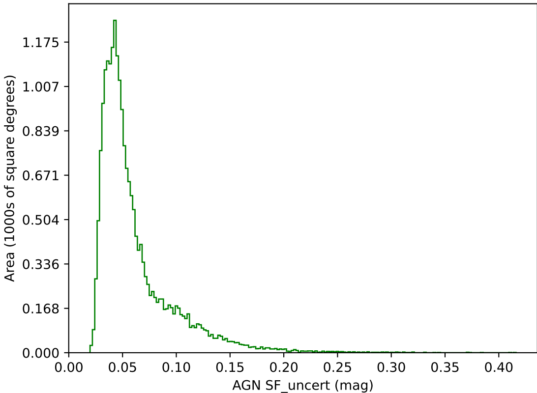
too_combined_s1.0_v3.4_10yrs g band: AGN SF_uncert
