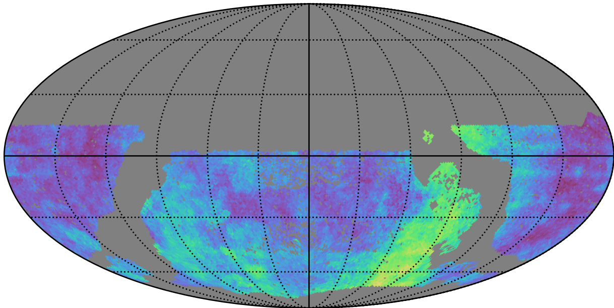
too_combined_s1.0_v3.4_10yrs WFD: Parallax Coverage @ 22.4
