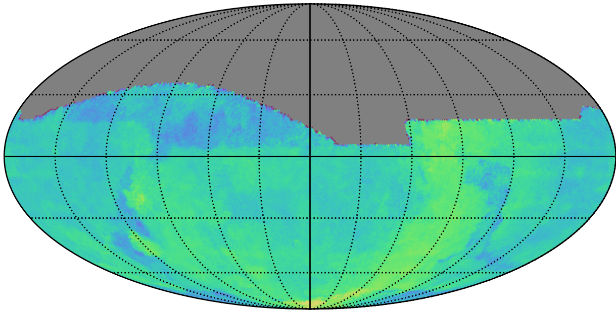
too_combined_s1.0_v3.4_10yrs All sky: Parallax Coverage @ 22.4
