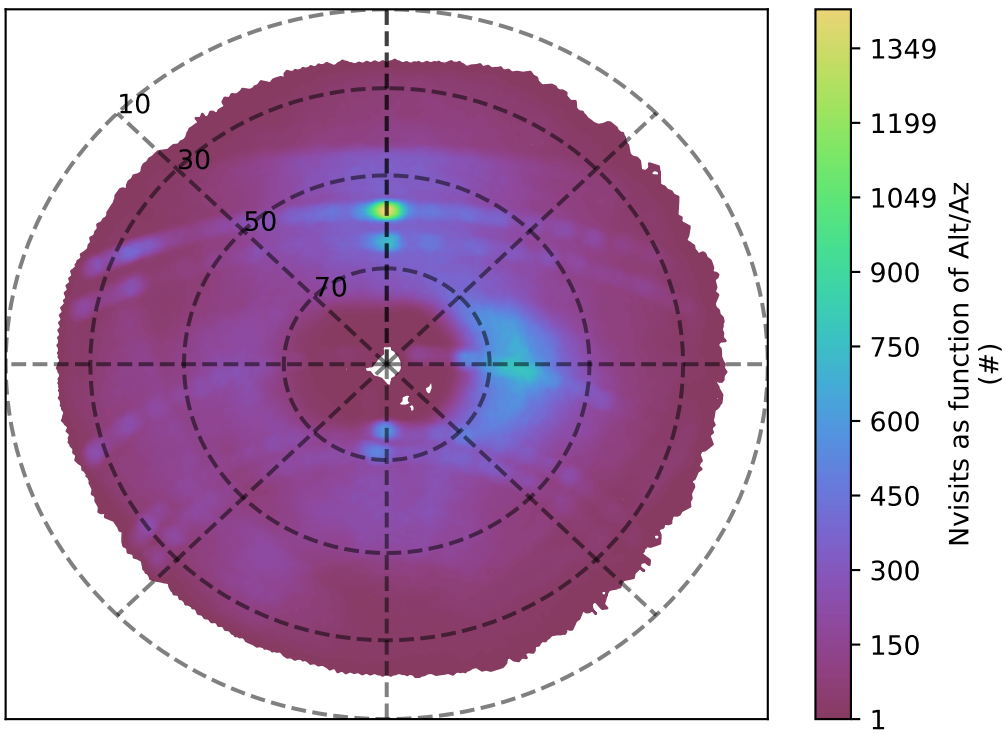
too_combined_s1.0_v3.4_10yrs g band: Nvisits as function of Alt/Az
