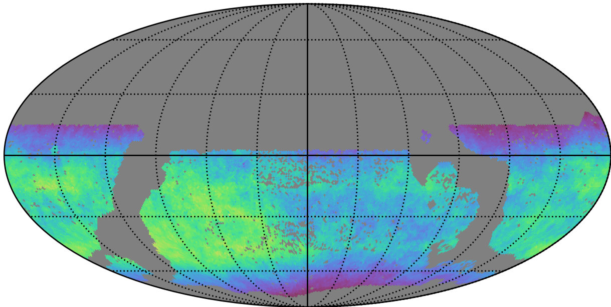
too_combined_s1.0_v3.4_10yrs WFD i band: Normalized Teff
