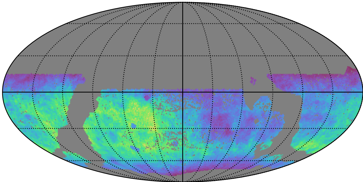
too_combined_s1.0_v3.4_10yrs WFD g band: Normalized Teff
