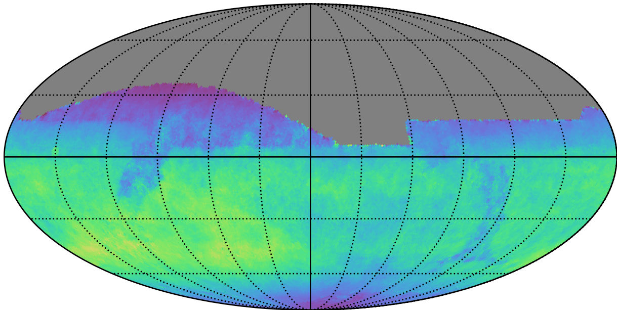
too_combined_s1.0_v3.4_10yrs All sky z band: Normalized Teff
