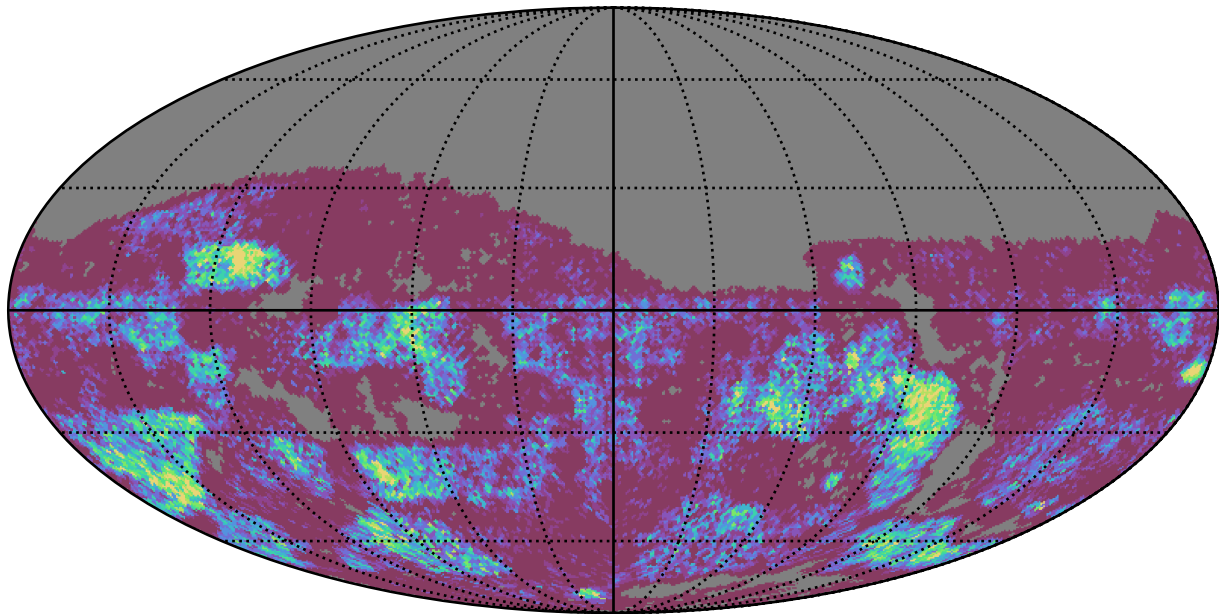
too_combined_s1.0_v3.4_10yrs Yr 3-4 g band: NVisits
