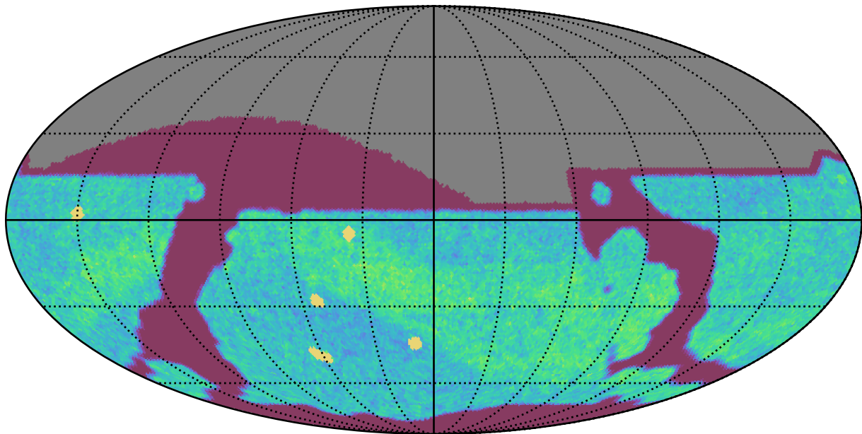
too_combined_s1.0_v3.4_10yrs All sky i band: NVisits
