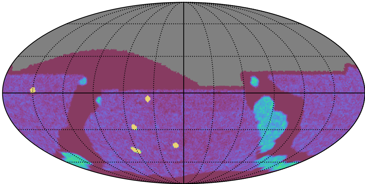
too_combined_s1.0_v3.4_10yrs All sky g band: NVisits
