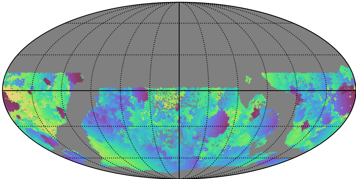
too_combined_s1.0_v3.4_10yrs WFD g band: Min solarElong
