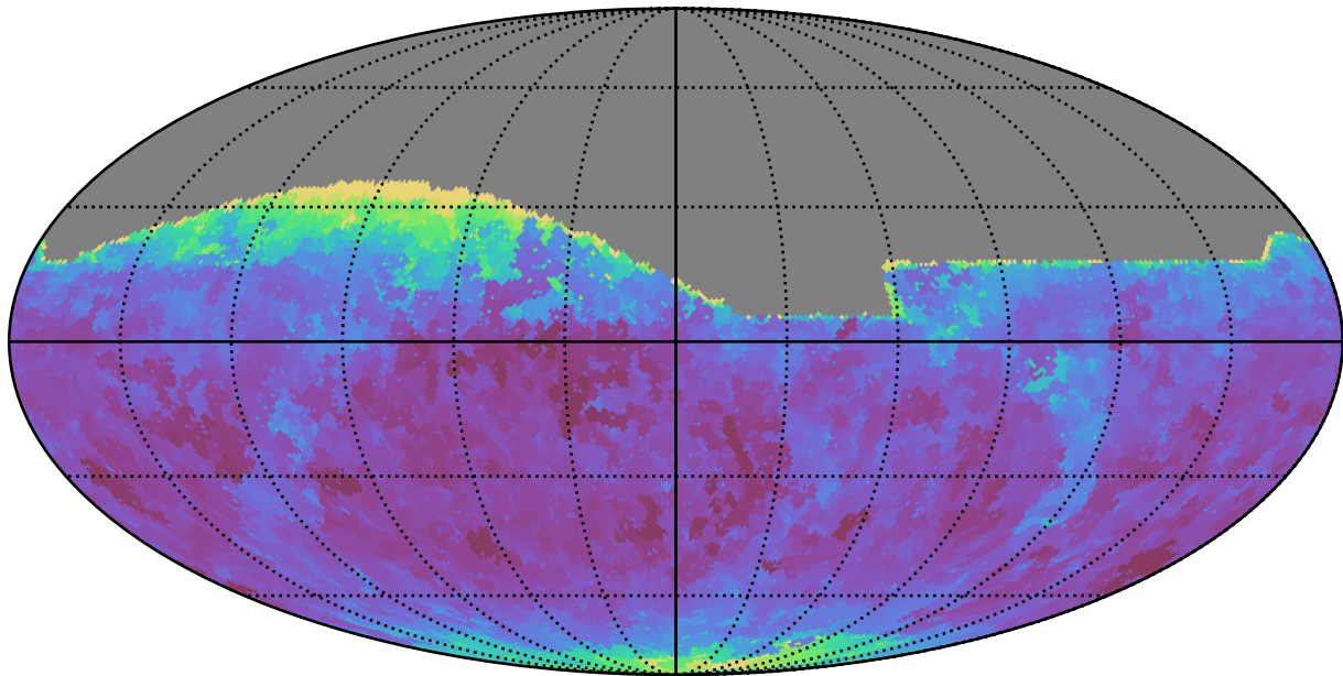
too_combined_s1.0_v3.4_10yrs All sky z band: Min seeingEff
