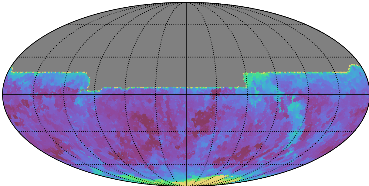
too_combined_s1.0_v3.4_10yrs All sky y band: Min seeingEff
