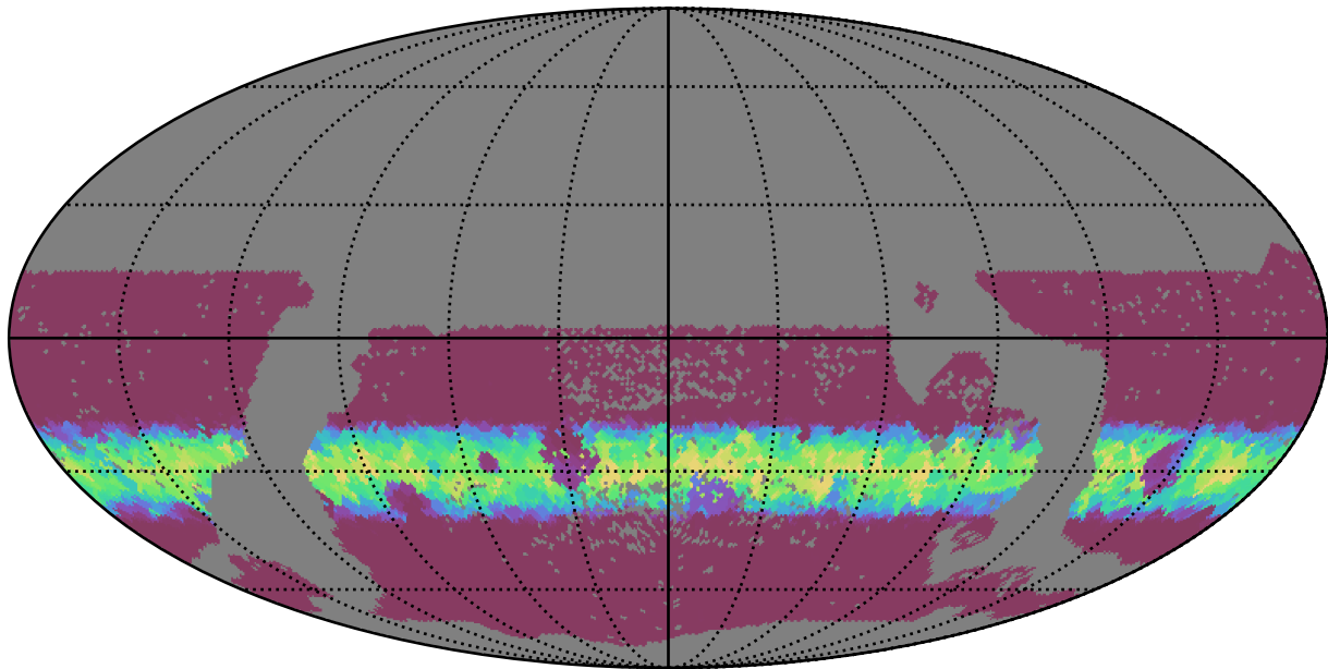
too_combined_s1.0_v3.4_10yrs WFD i band: Min normairmass
