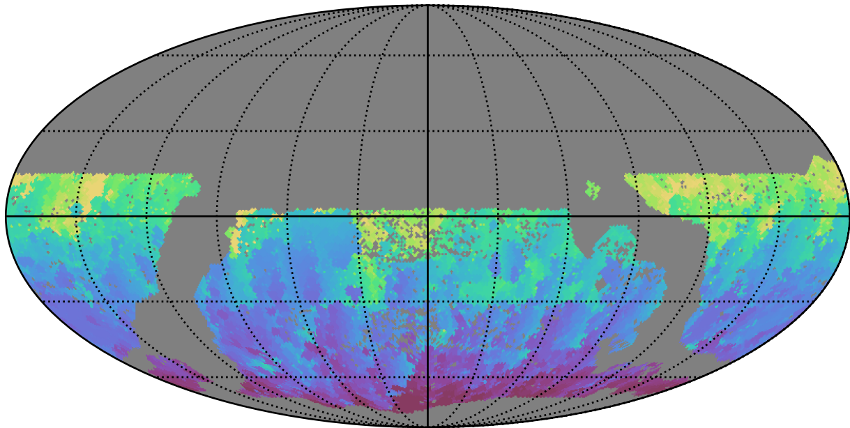
too_combined_s1.0_v3.4_10yrs WFD g band: Min HA
