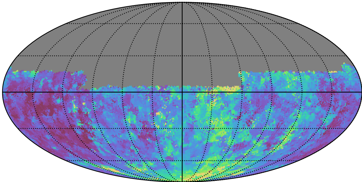
too_combined_s1.0_v3.4_10yrs Yr 1 u band: Median seeingEff
