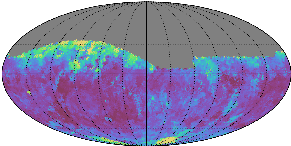
too_combined_s1.0_v3.4_10yrs Yr 1 i band: Median seeingEff
