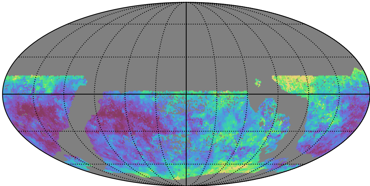
too_combined_s1.0_v3.4_10yrs WFD u band: Median seeingEff
