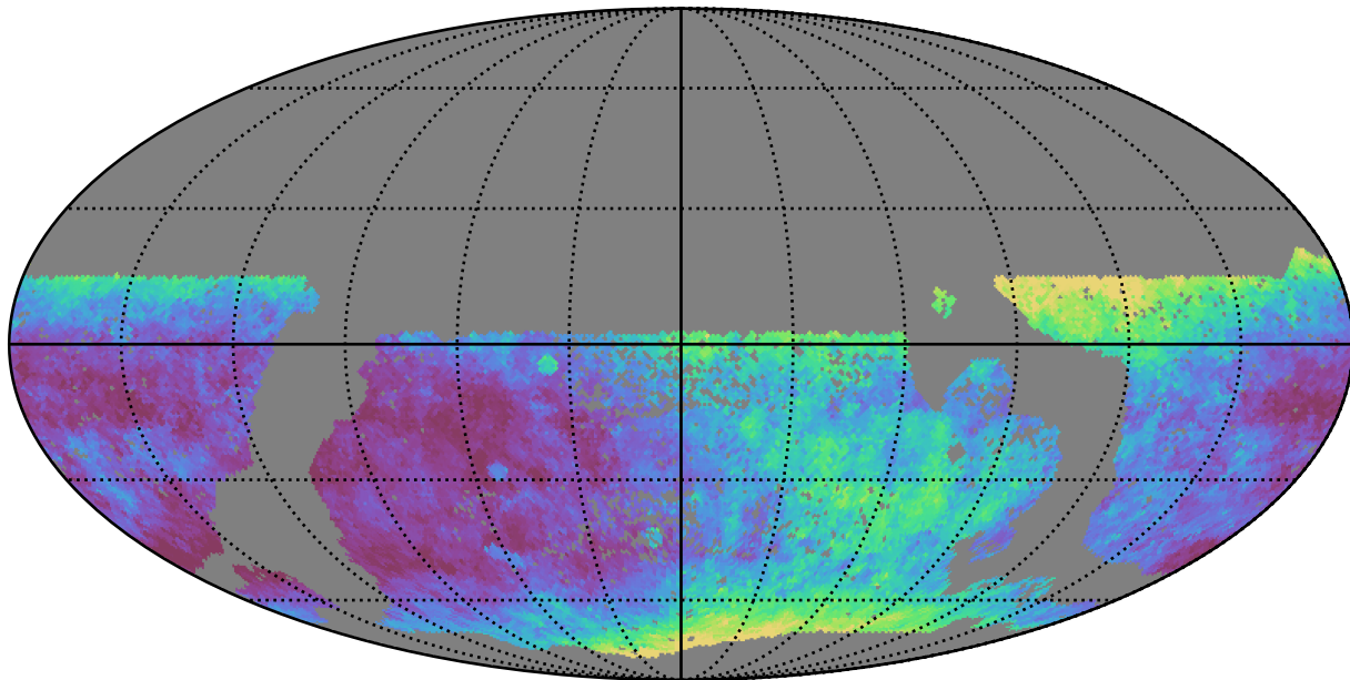
too_combined_s1.0_v3.4_10yrs WFD r band: Median seeingEff
