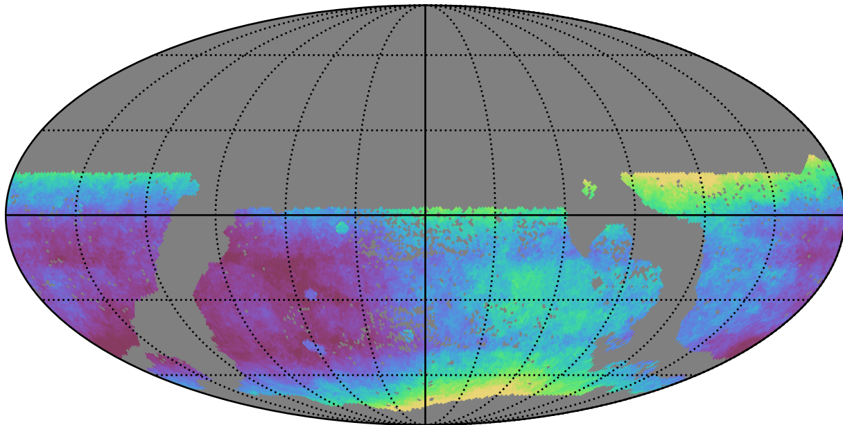
too_combined_s1.0_v3.4_10yrs WFD all bands: Median seeingEff
