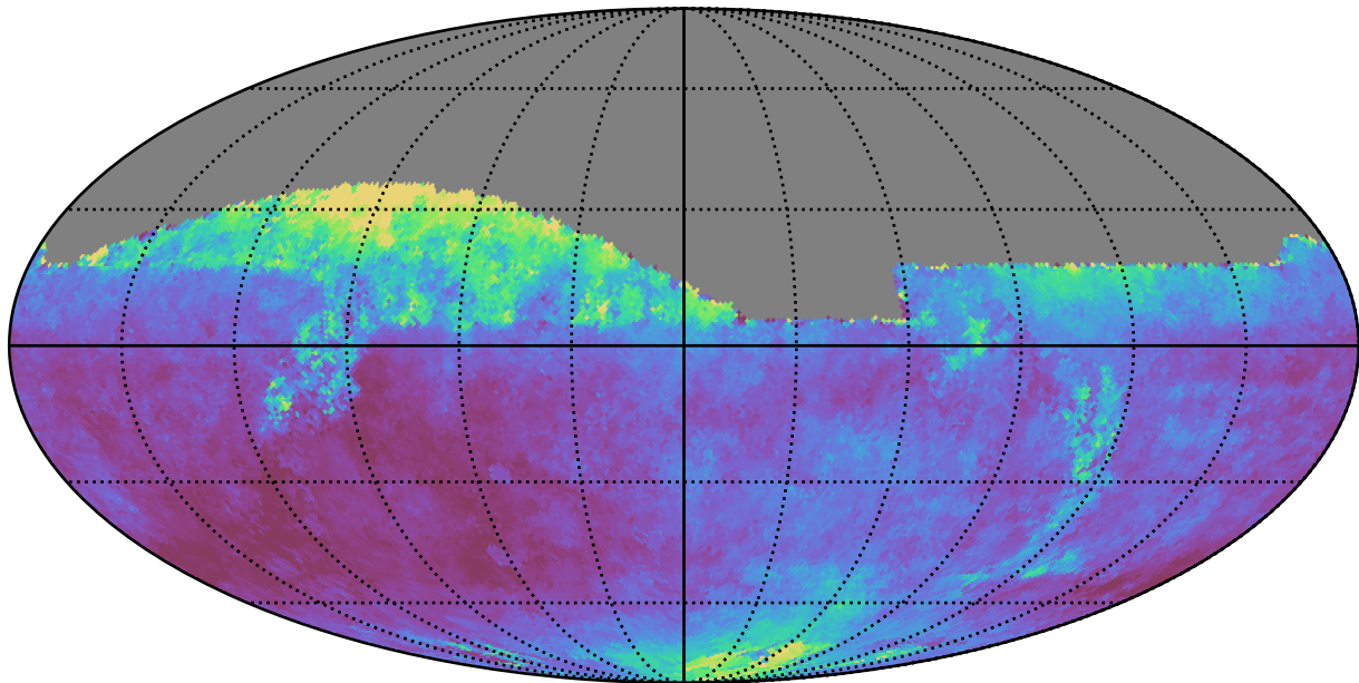
too_combined_s1.0_v3.4_10yrs All sky z band: Median seeingEff
