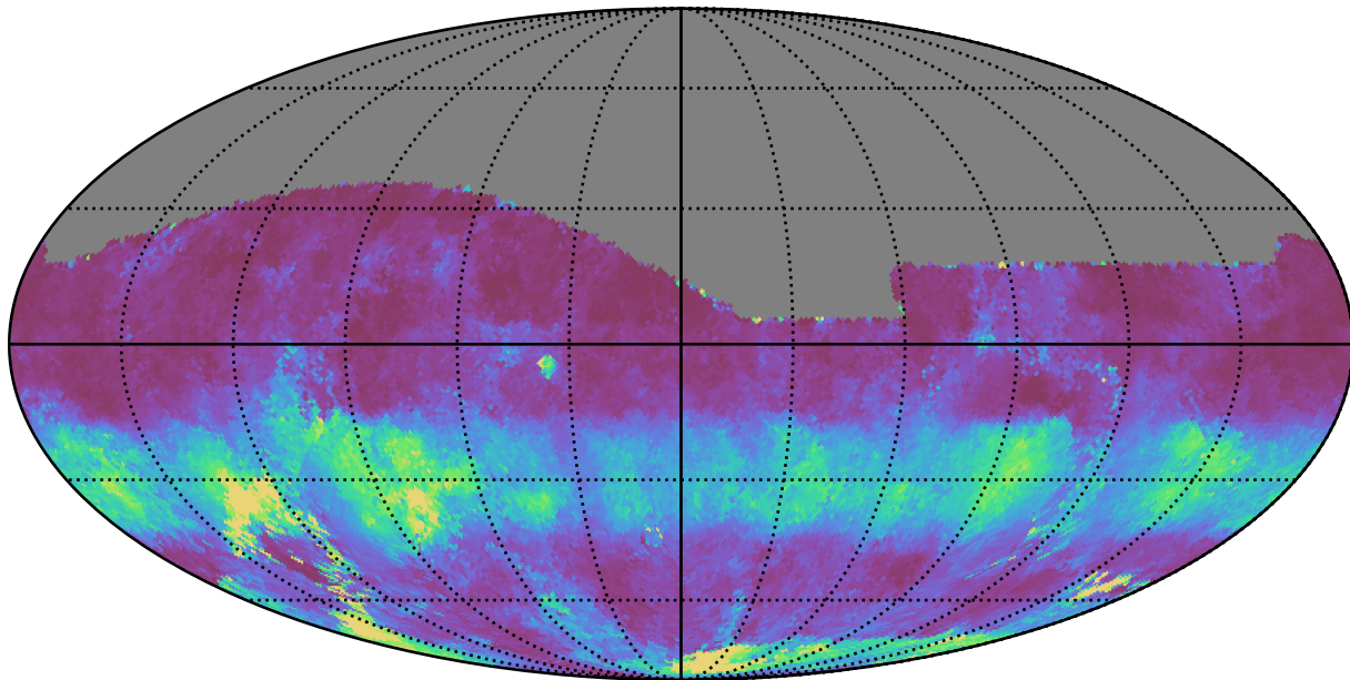
too_combined_s1.0_v3.4_10yrs All sky g band: Median normairmass
