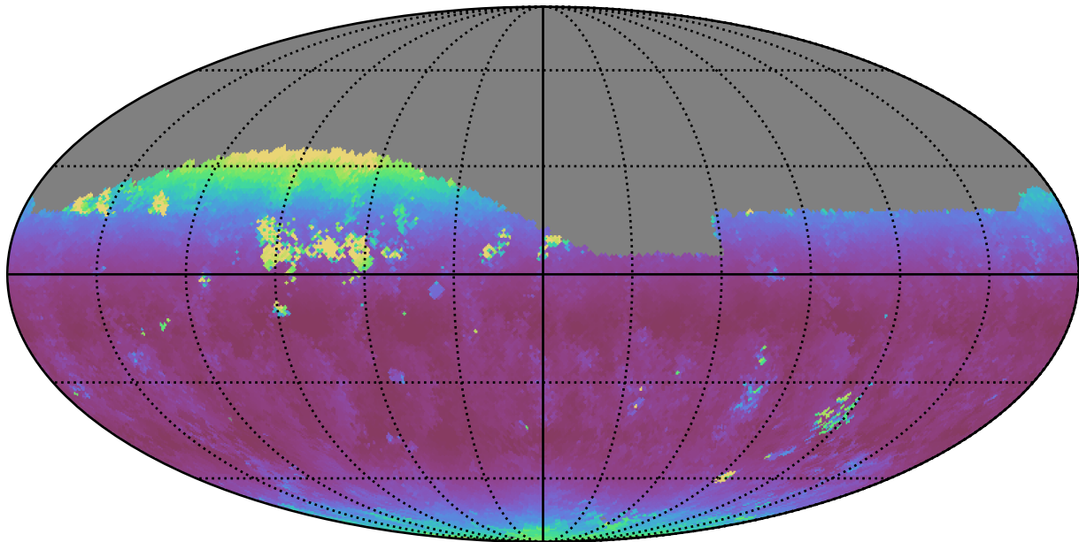
too_combined_s1.0_v3.4_10yrs Yr 1 z band: Median airmass
