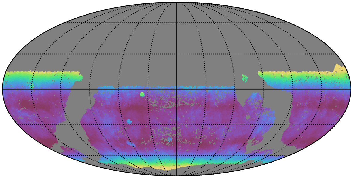
too_combined_s1.0_v3.4_10yrs WFD y band: Median airmass
