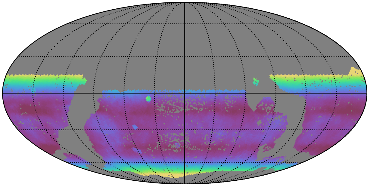
too_combined_s1.0_v3.4_10yrs WFD all bands: Median airmass
