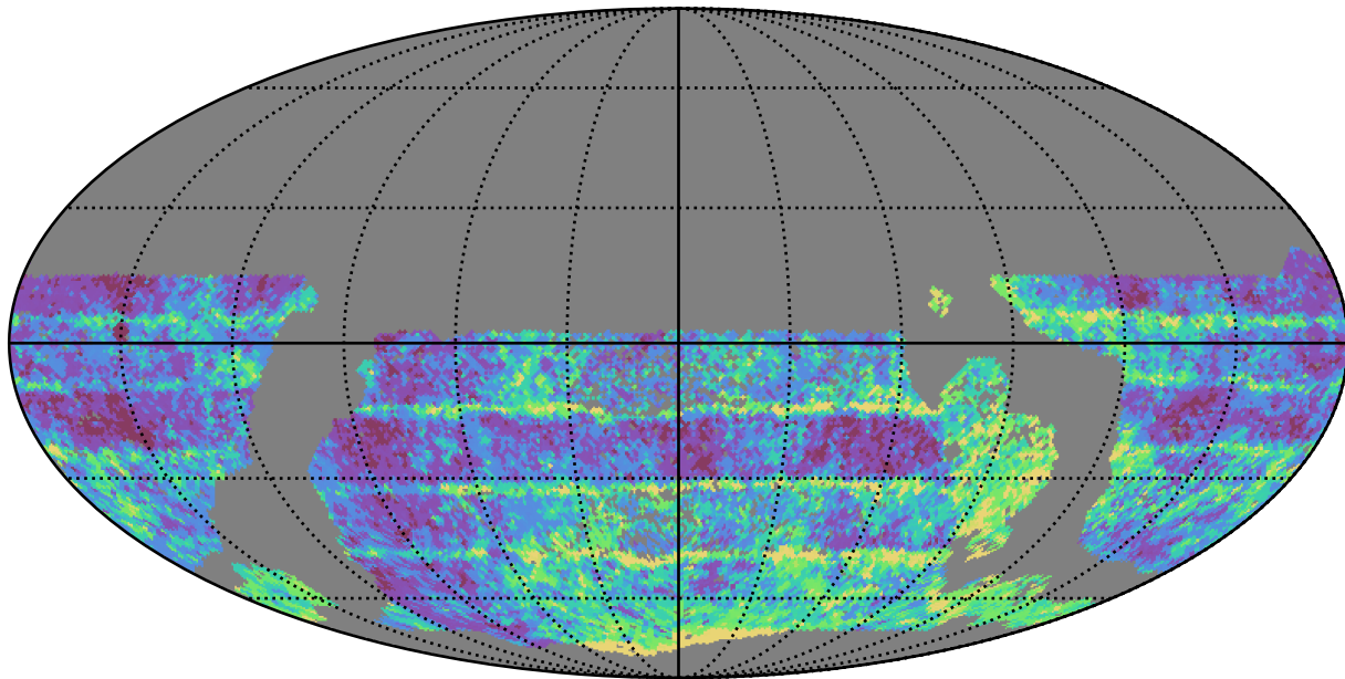
too_combined_s1.0_v3.4_10yrs WFD r band: Median Inter-Night Gap
