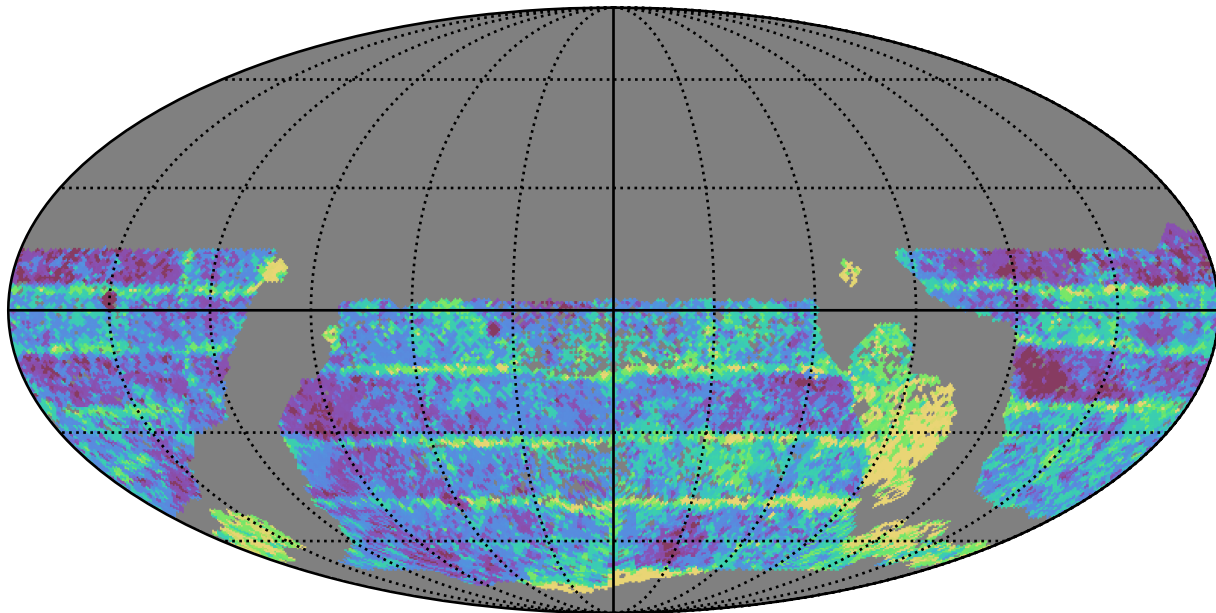
too_combined_s1.0_v3.4_10yrs WFD i band: Median Inter-Night Gap
