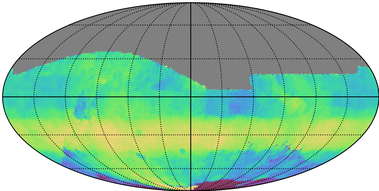
too_combined_s1.0_v3.4_10yrs All sky r band: Median HA
