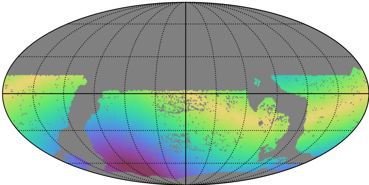
too_combined_s1.0_v3.4_10yrs WFD u band: Max solarElong
