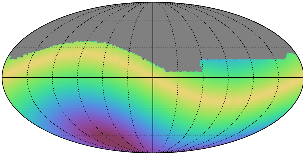
too_combined_s1.0_v3.4_10yrs All sky all bands: Max solarElong
