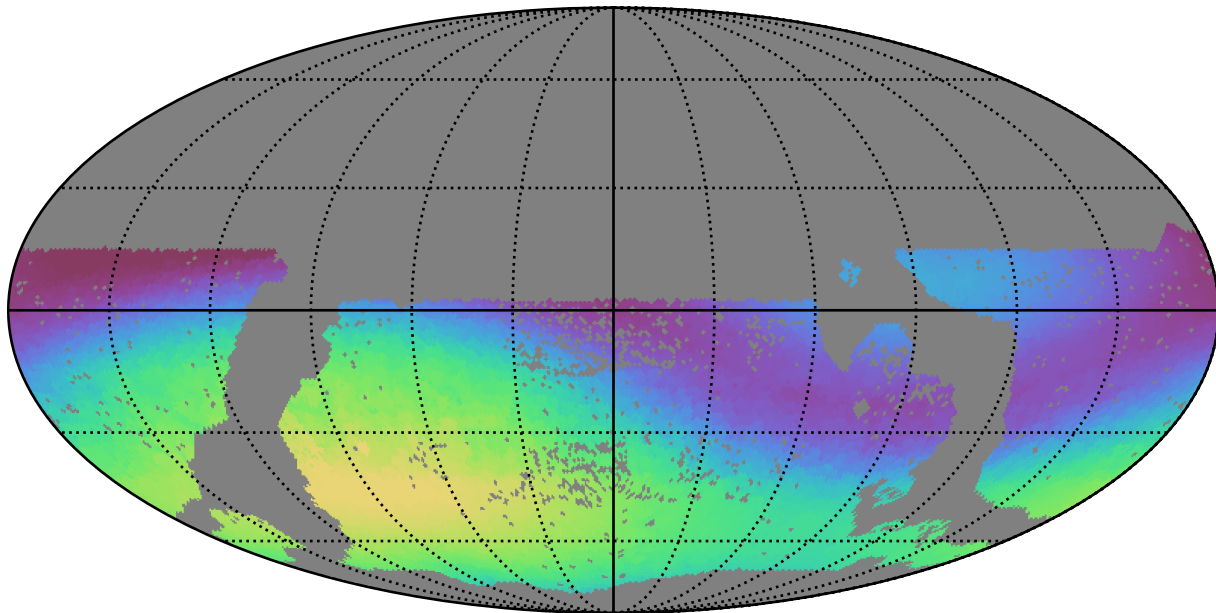
too_combined_s1.0_v3.4_10yrs WFD g band: Max skyBrightness
