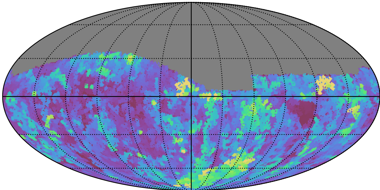
too_combined_s1.0_v3.4_10yrs Yr 1 g band: Max seeingGeom
