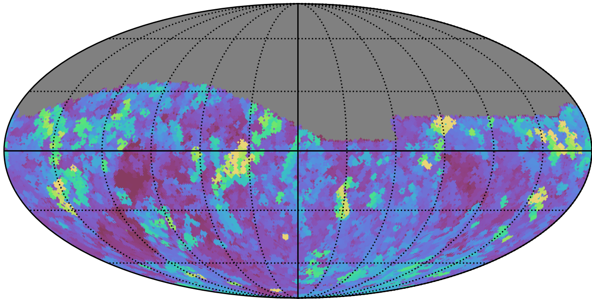
too_combined_s1.0_v3.4_10yrs Yr 1 z band: Max seeingEff
