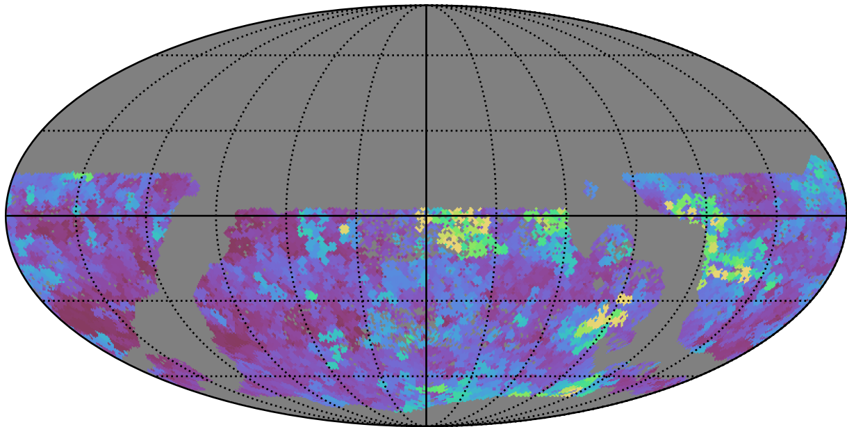
too_combined_s1.0_v3.4_10yrs WFD y band: Max seeingEff
