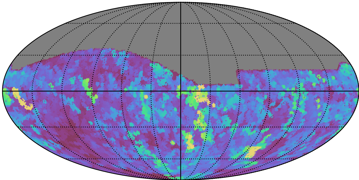
too_combined_s1.0_v3.4_10yrs All sky z band: Max seeingEff
